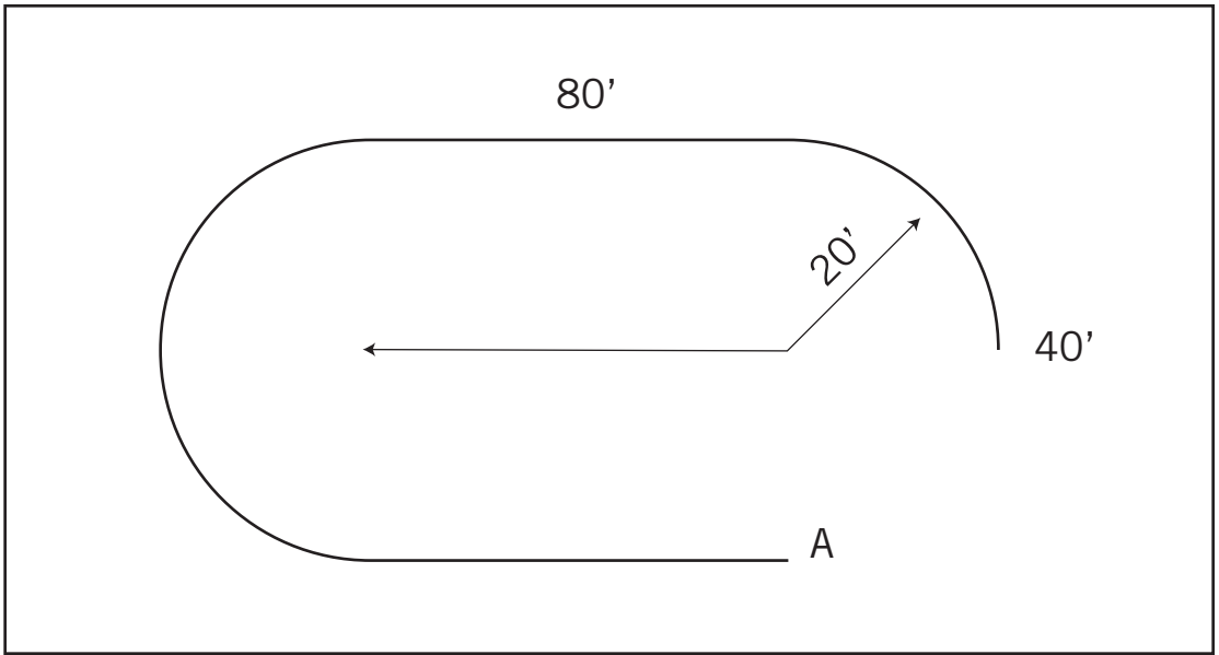
Figure 7b. Establishing Tent Perimeter—Round-End Tent
