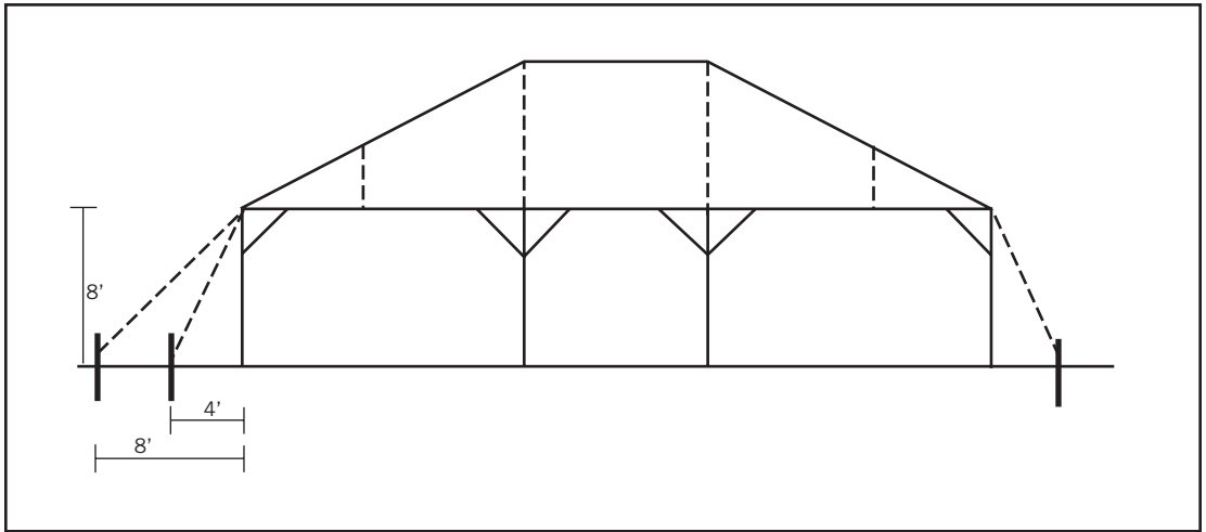
Figure 45. Suggested Guy-Rope Angle for Typical Frame Tent
