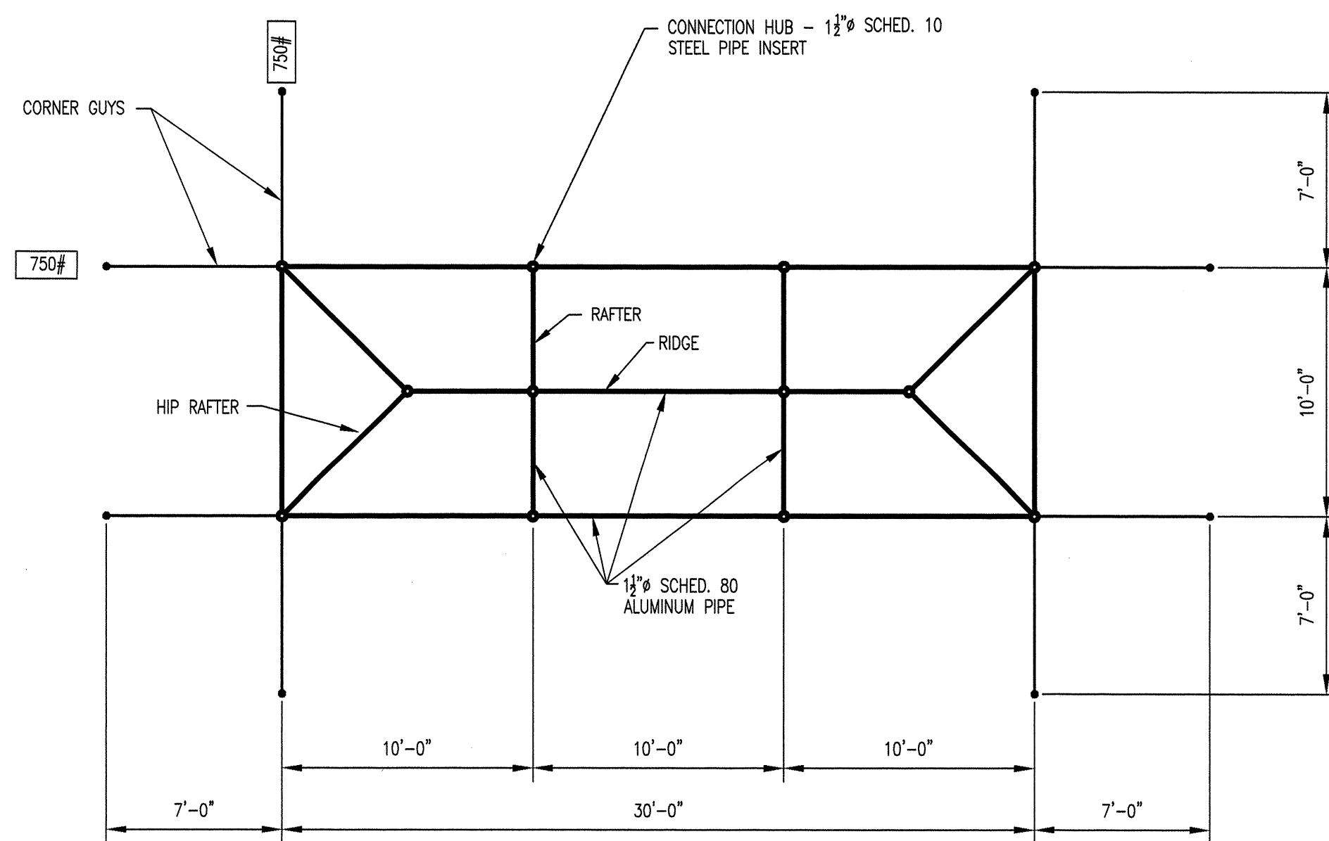
PLAN
