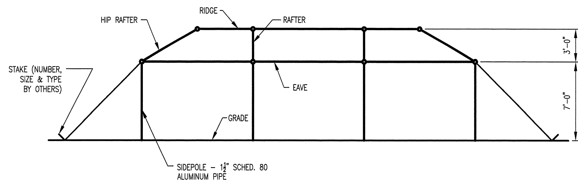
SIDE ELEVATION
