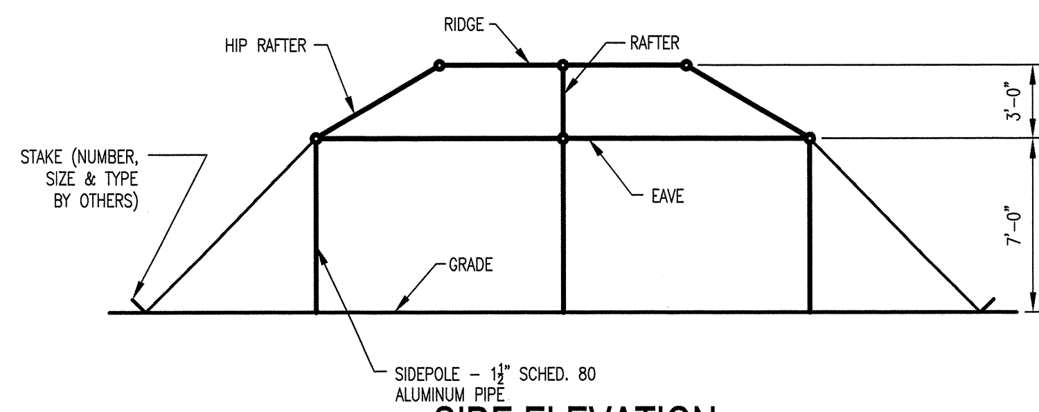
SIDE ELEVATION
