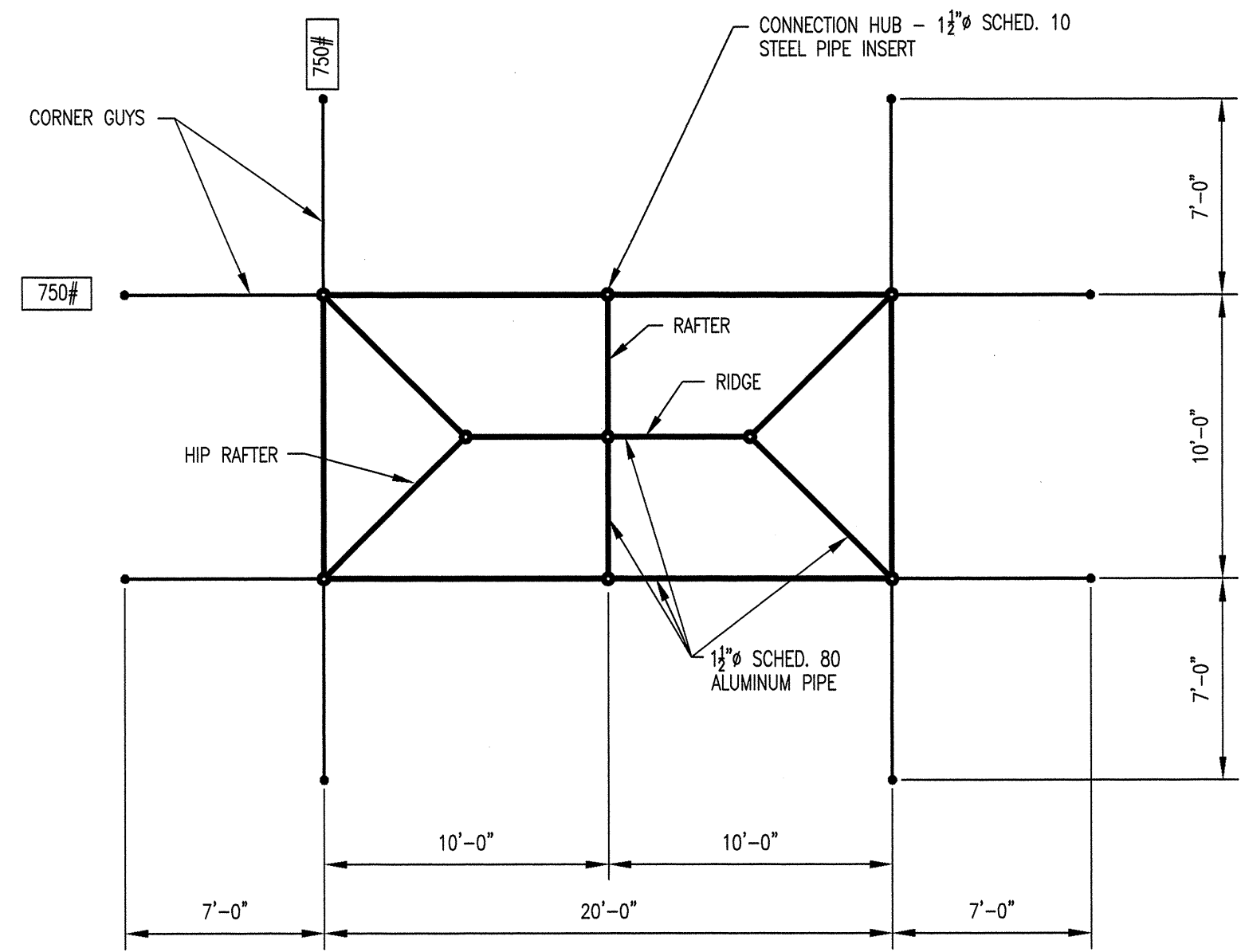
PLAN
