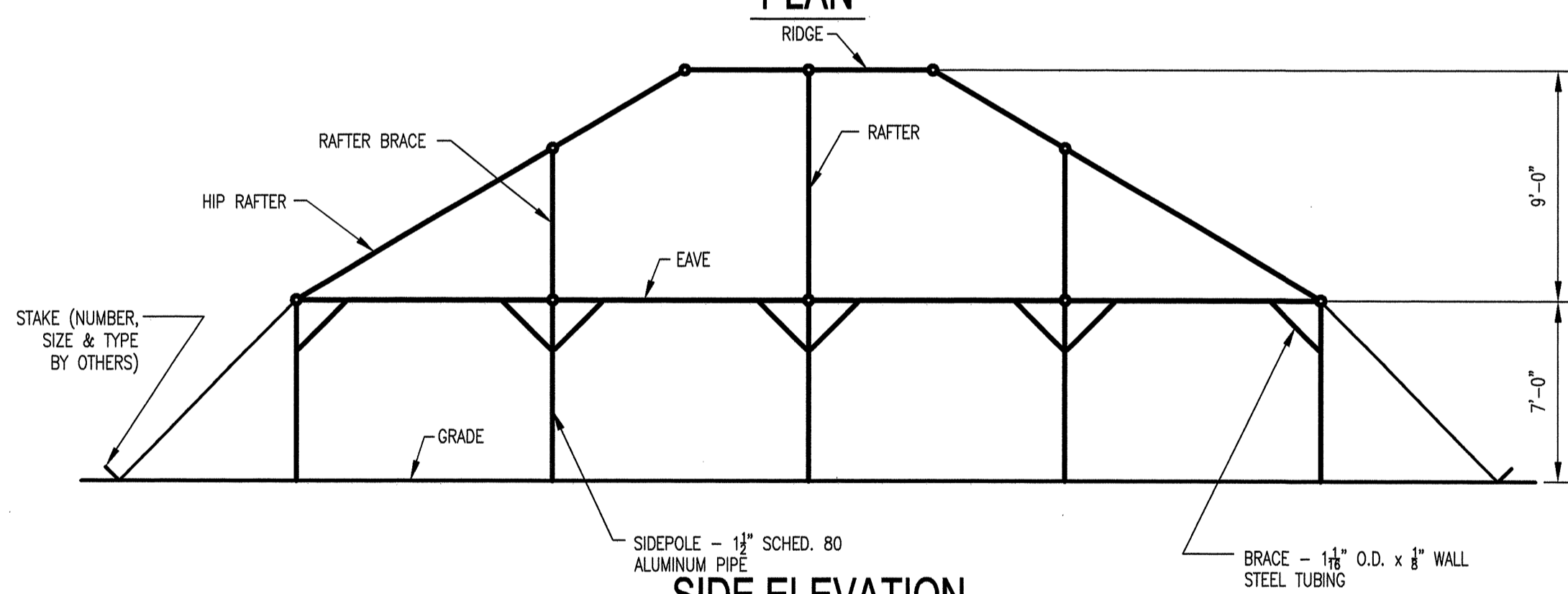
SIDE ELEVATION
