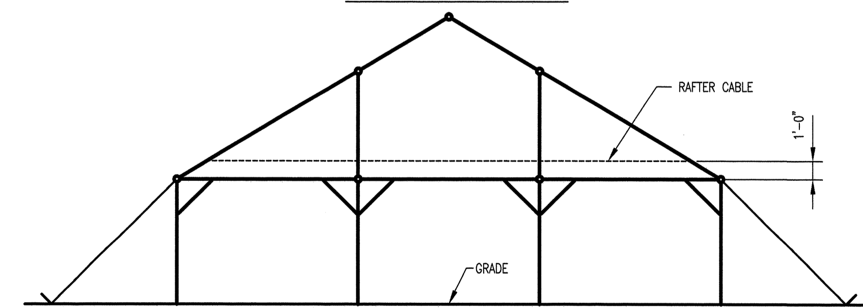
SIDE ELEVATION
