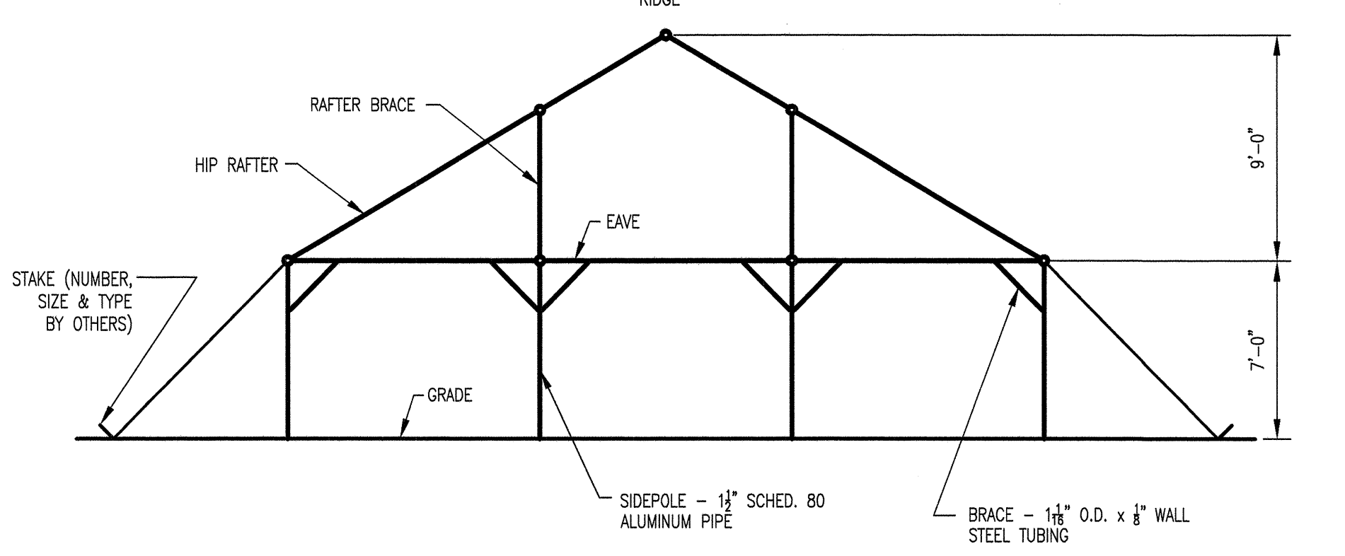
SIDE ELEVATION
