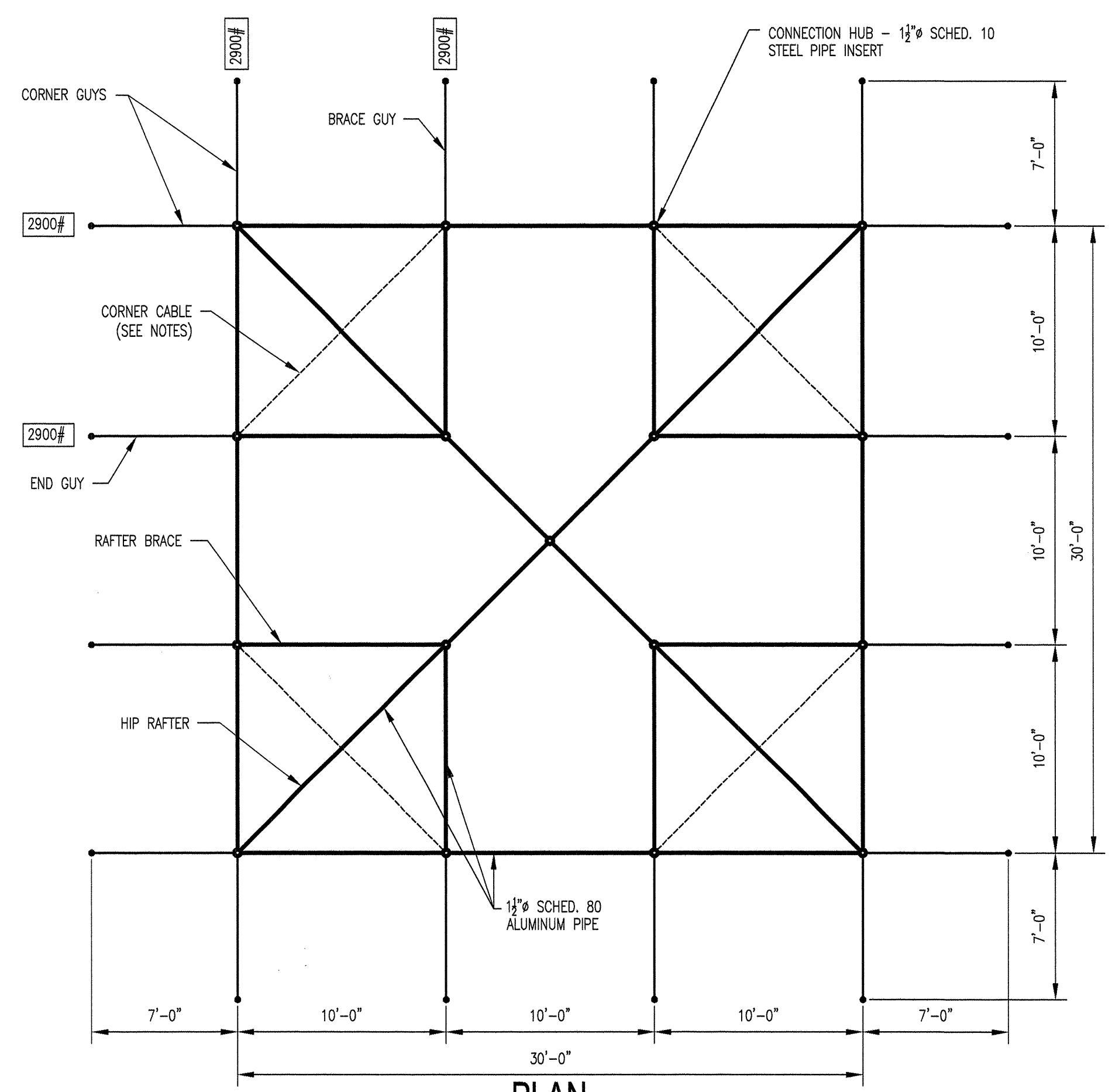
PLAN
