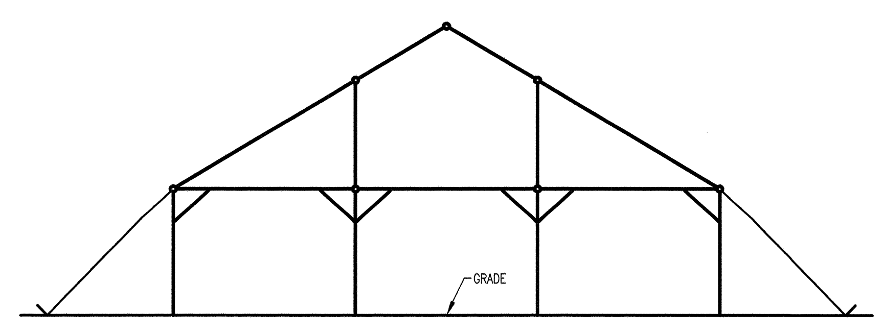
END ELEVATION 30' WIDE CELEBRATION
