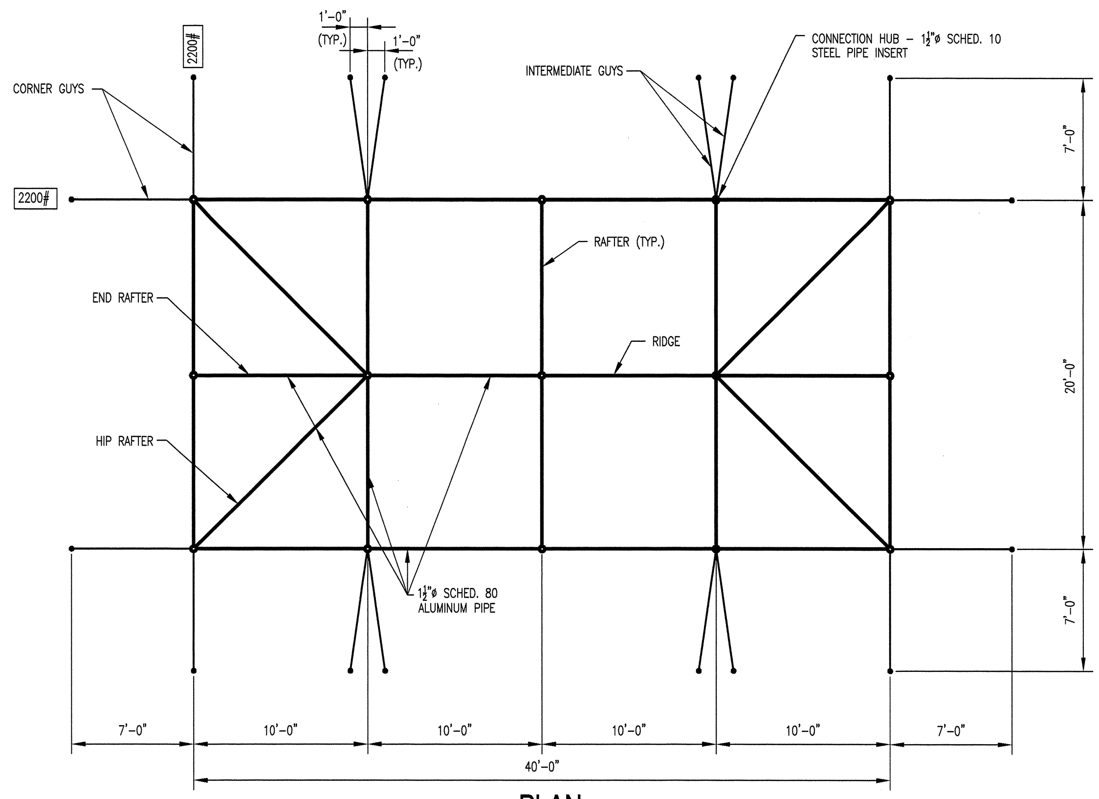
PLAN
