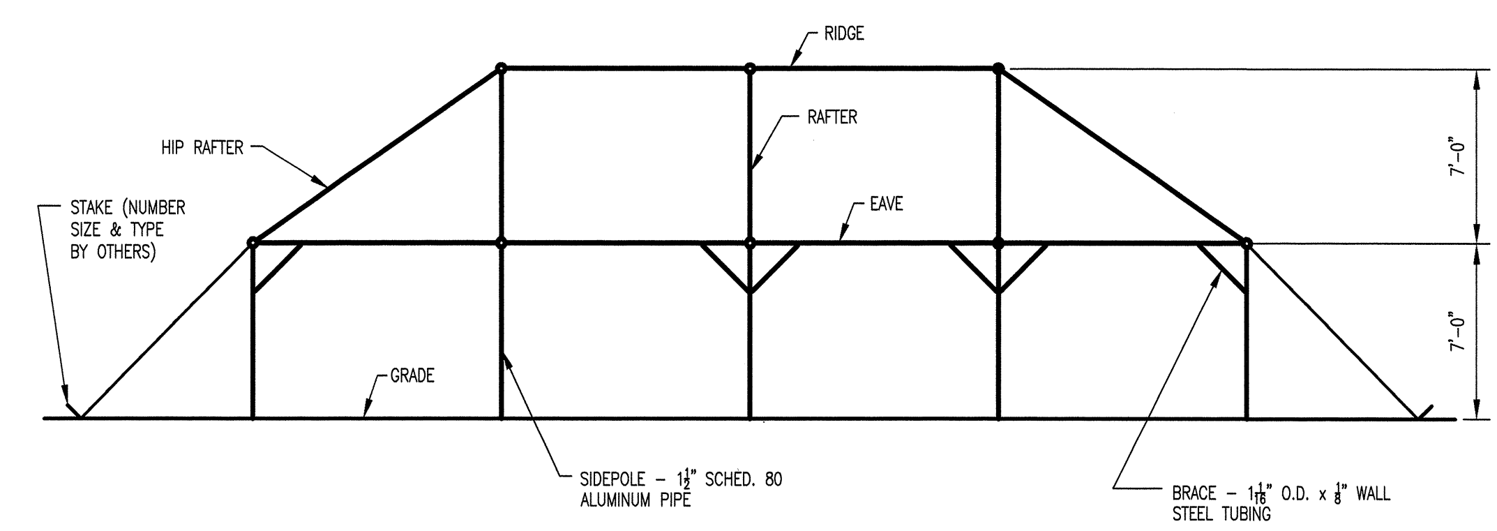
SIDE ELEVATION
