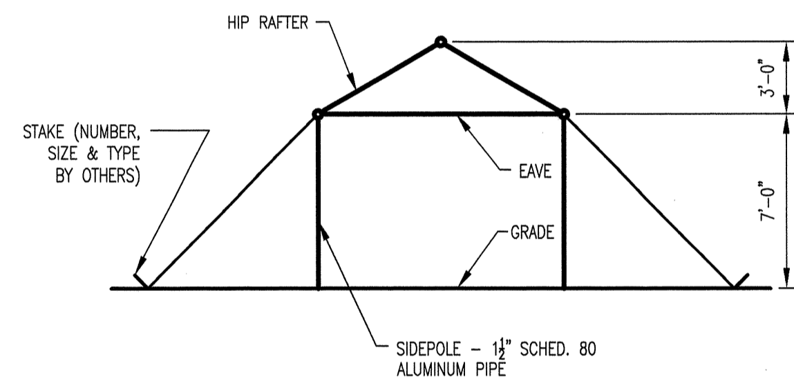
SIDE ELEVATION
