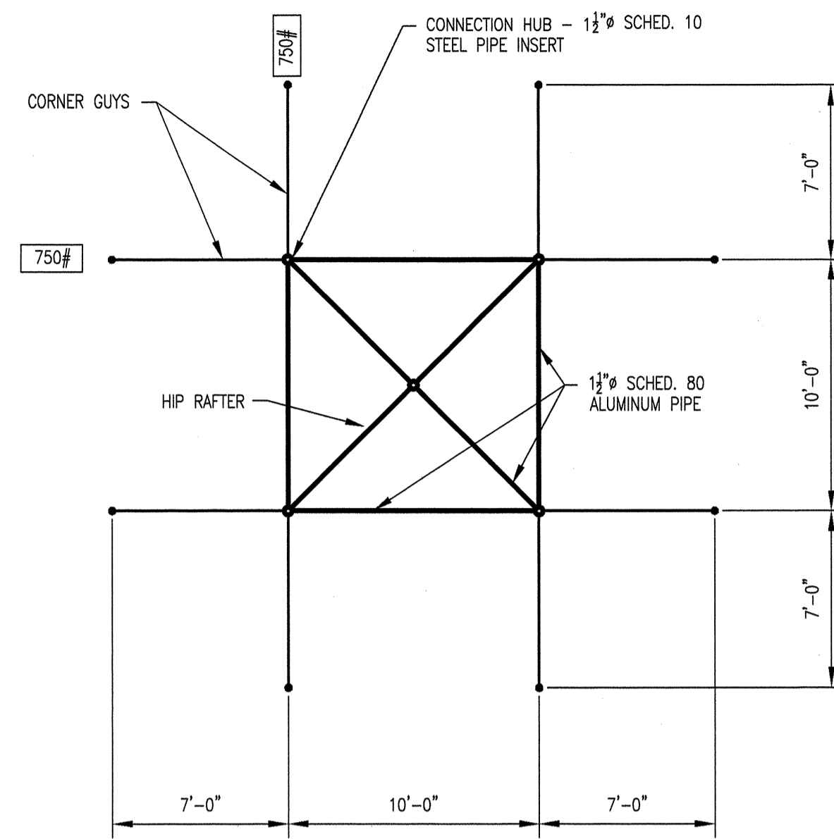
PLAN
